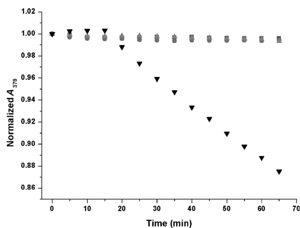
Figure 2. Relative ^1O_2 -generation efficiency of micellar Gate 1 (7.5 \mu M) in aqueous solutions in the presence (▼) or absence (▲) of acid, detected by the absorption decrease of the trap at 378 nm. The changes in the trap absorption in slightly basic (■) and acidic (●) solutions (pH = ca. 7.5 and 6.0, respectively) are also shown. During the first 15 min, the samples were kept in the dark, and for the following 50 min, the samples were irradiated with 660 nm light using an LED array.
